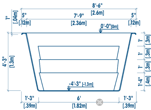
CORTE TRANSVERSAL | CROSS SECTION
